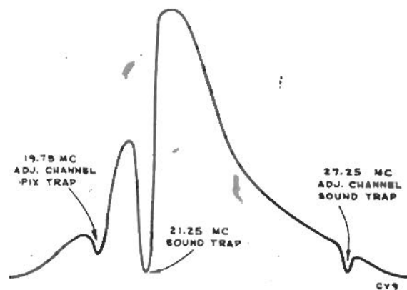
Figure 30—T2 Response
