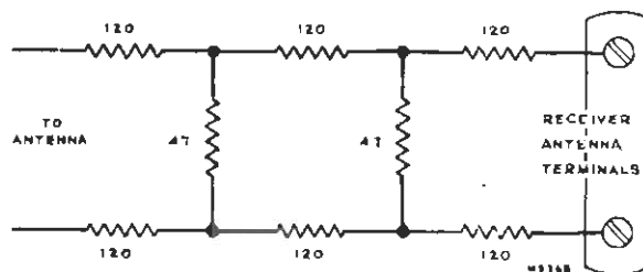
Figure 13—Attenuator Pad
