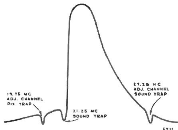
Figure 32—T104 Response
