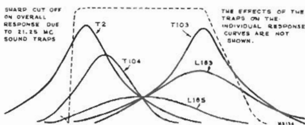
Figure 3—Stagger Tuned I-F Response
