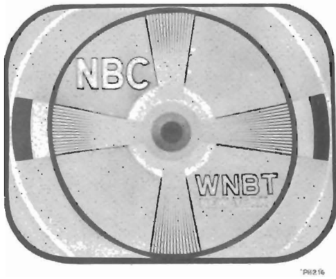
Figure 44—Focus Coil and Ion Trap Magnet Misadjusted
