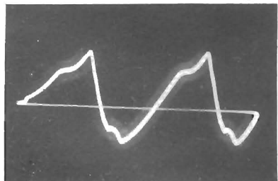
Figure 104—Plate of Horizontal Output (Approx. 6000 Volts PP) (Measured Through a Capacity Voltage Divider Connected from Top Cap of V126 to Ground)
