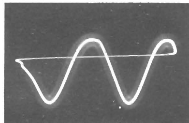
Figure 98—Cathode of Horizontal Oscillator Control (1.5 Volts PP) (Pin 5 of V124) (6AC7)
