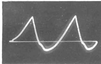
Figure 101—Plate of Hor. Discharge (78 Volts PP) (Pin 5 of V120-B) (6SN7GT)
