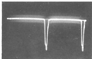
Figure 105—Cathode of Reaction Scanning (60 Volts PP) (Pin 8 of V128) (5V4G)
