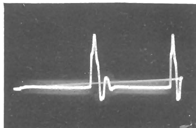
Figure 103—Screen of Hor. Output (9 Volts PP) (Pin 8 of V126) (6BG6-G)
