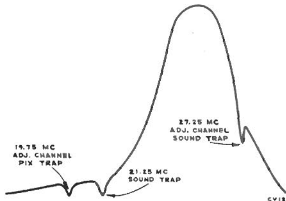
Figure 33—L183 Response
