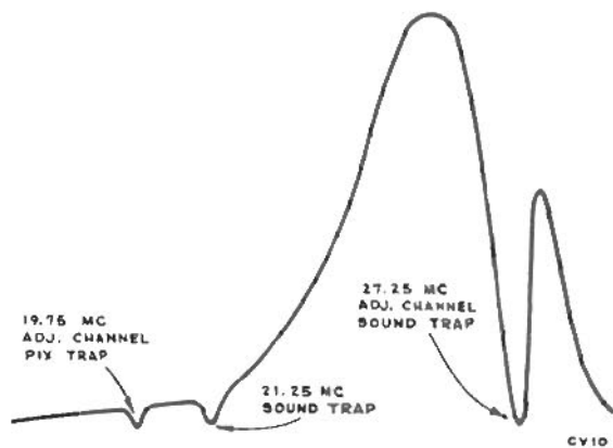
Figure 31—T103 Response
