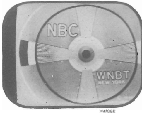
Figure 47—Horizontal Centering Control Misadjusted
